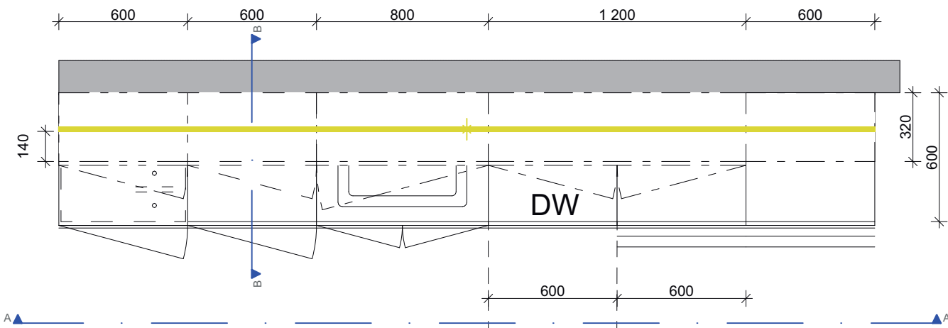
PLAN
