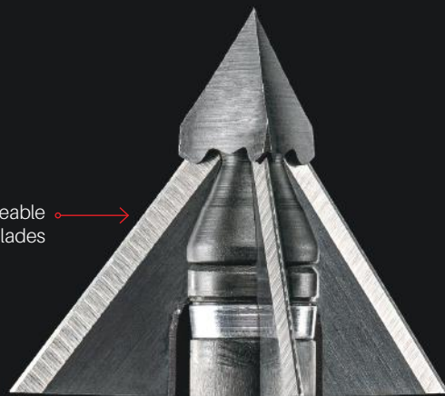
FULL BLADE
