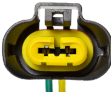
SOCKET SQ-580
