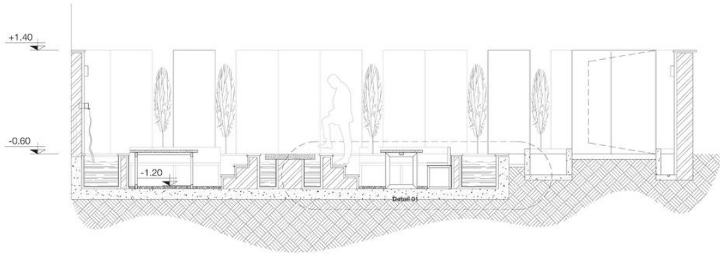
Section C-C
