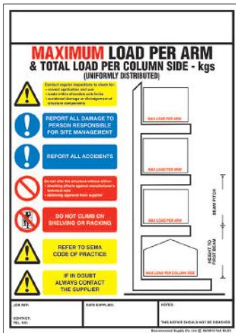
BLS2 Cantilever Racking (356mm x 254mm)
