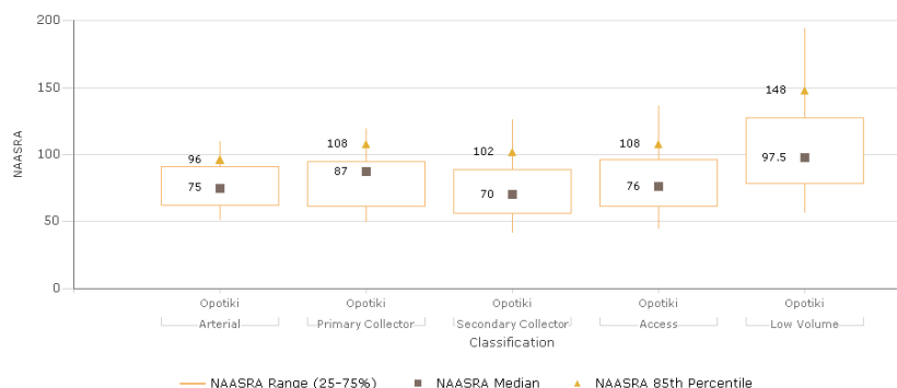
Figure 11-3: Average Roughness by ONRC
