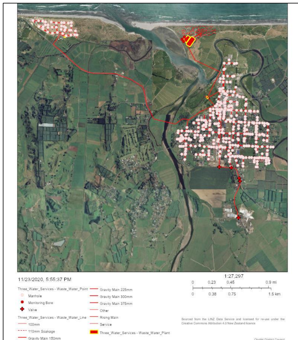
Figure 3 5 Wastewater Network extent for Ōpōtiki and the Waiotahi Drifts.
