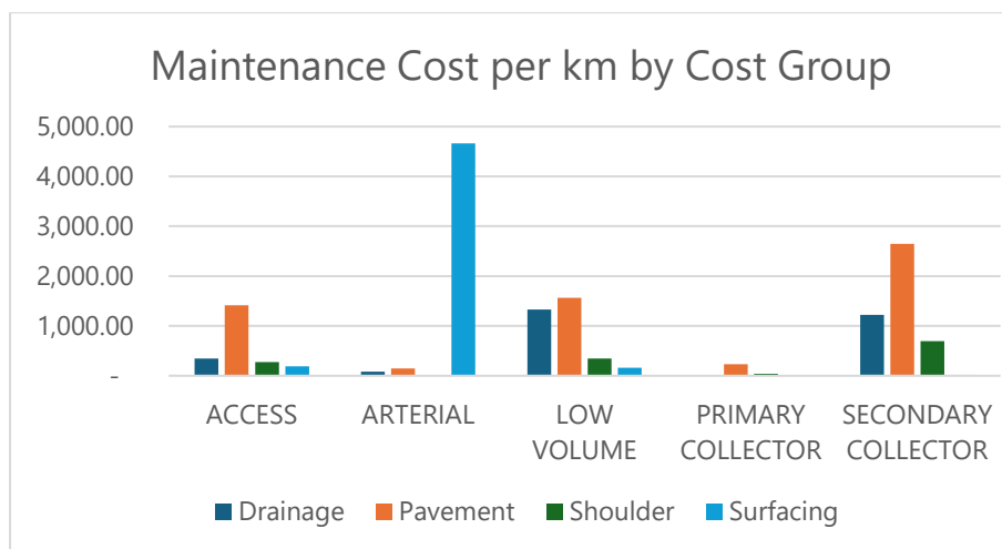
Figure 11-4: Maintenance Expenditure per km
