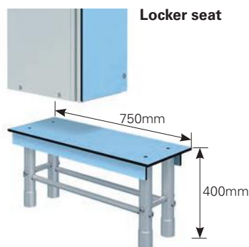
Locker seat
