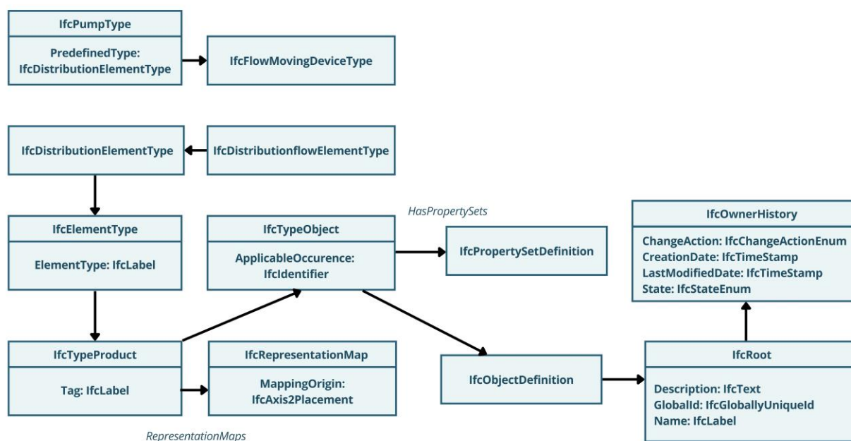
Figure 16 Data Schema from IFC 4.3 for a Pump
