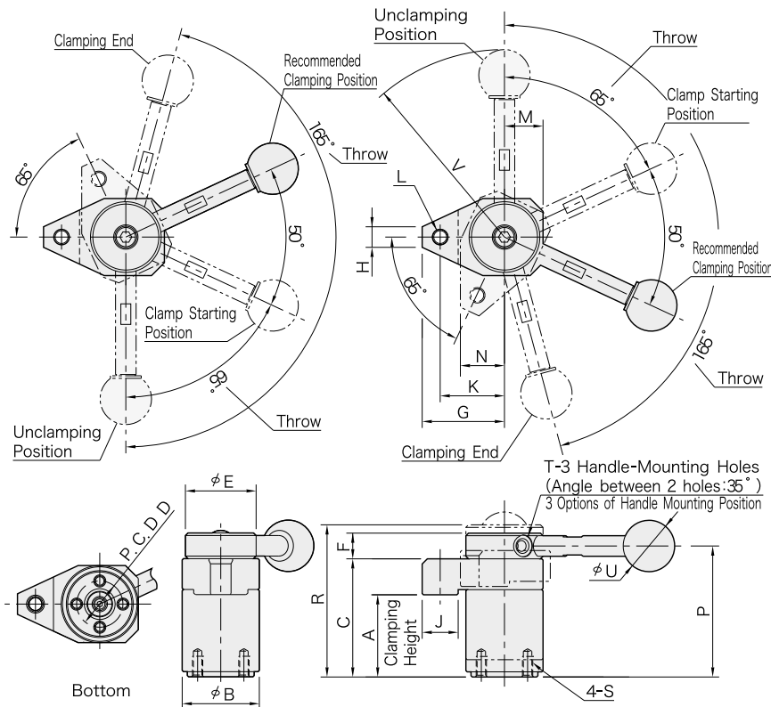
Counterclockwise Clamping
