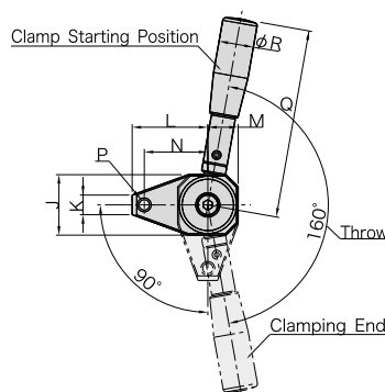
Clockwise Clamping
