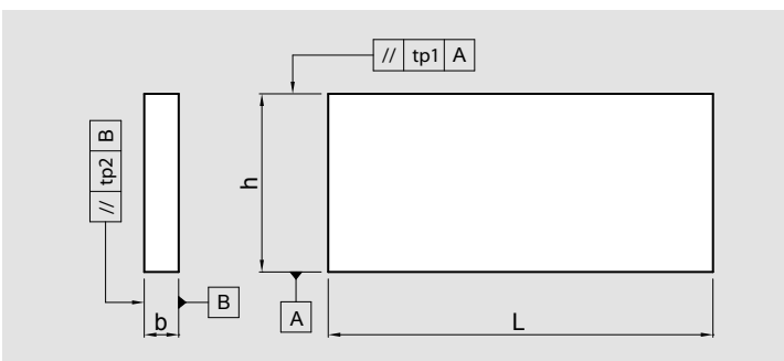
Set of 6 pairs of parallels (no clak) LC
