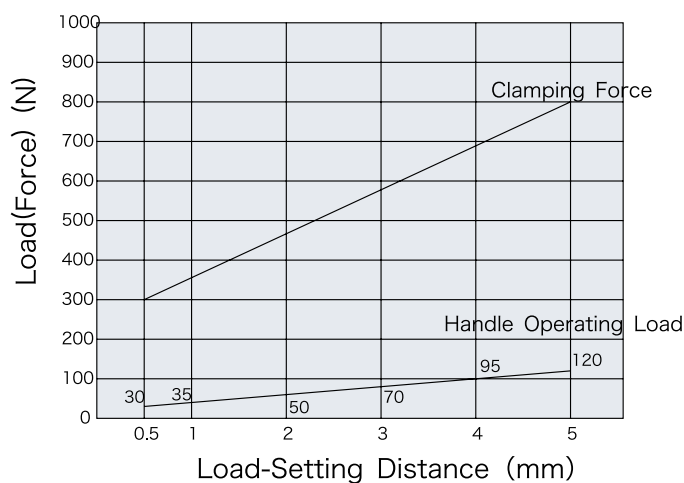
Swing Clamps (QLSW150)
