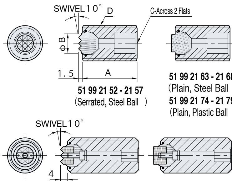
51 99 21 69 - 21 73 (Plain, Steel Tip)
