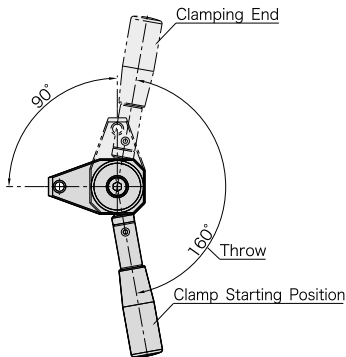
Counterclockwise Clamping
