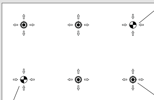
Type A Clamping pin with positioning accuracy
