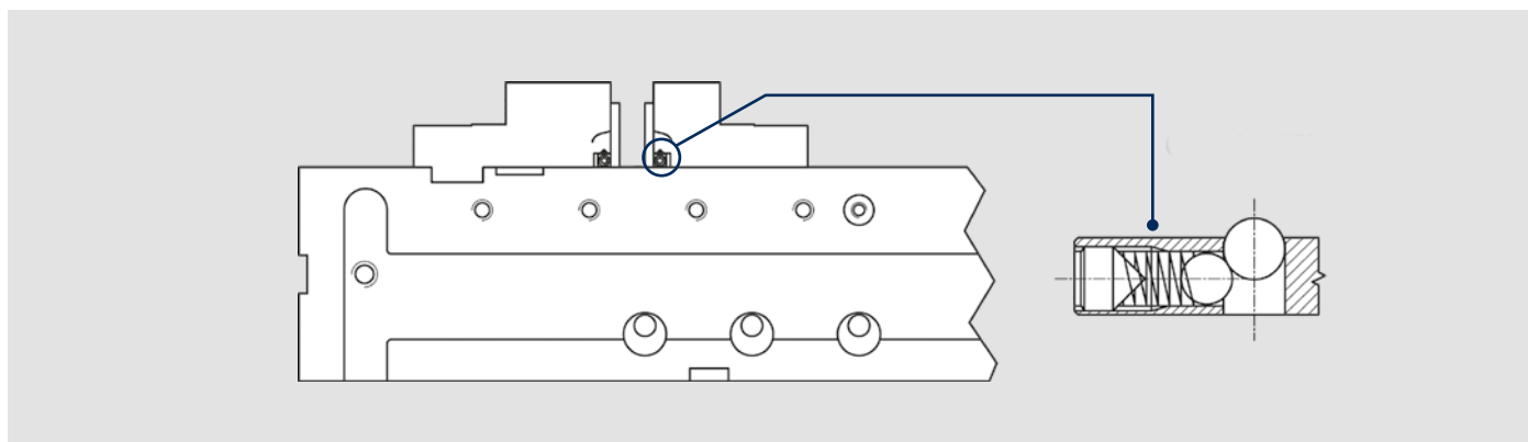
Universal CLAK System
