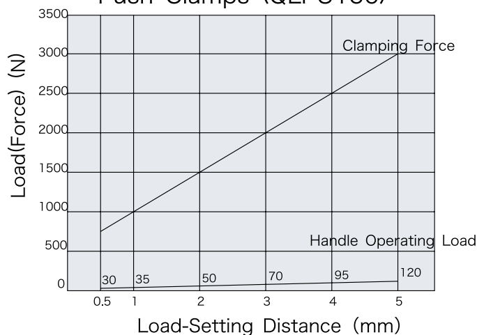
Side Clamps (QLSC150) Push Clamps (QLPU150)
