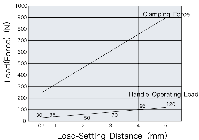
Pull Clamps (QLPD150)
