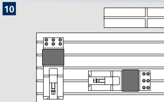
Cross key for T-slots M.T.
