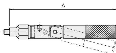
Plug-In Handle Coupled with the Adaptor
