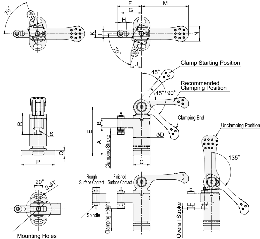
Counterclockwise Clamping
