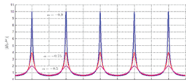
Comb filter
