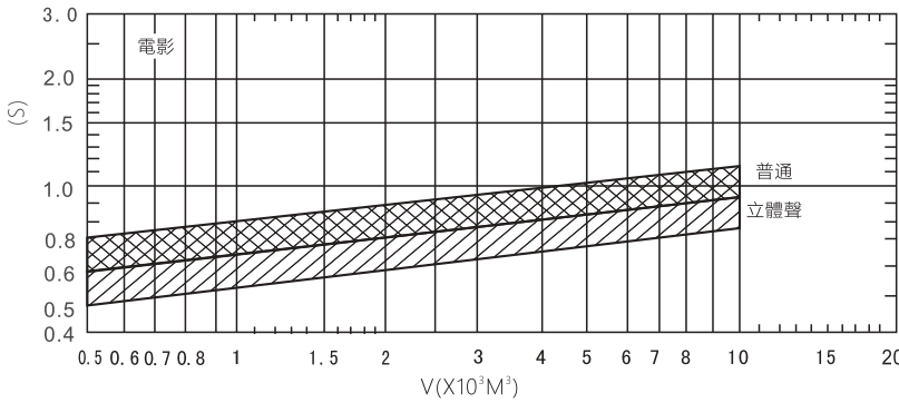
Figure 1 Range of proper reverberation time T for full cinema audience halls with different volumes V at 500 ~ 1000 Hz
