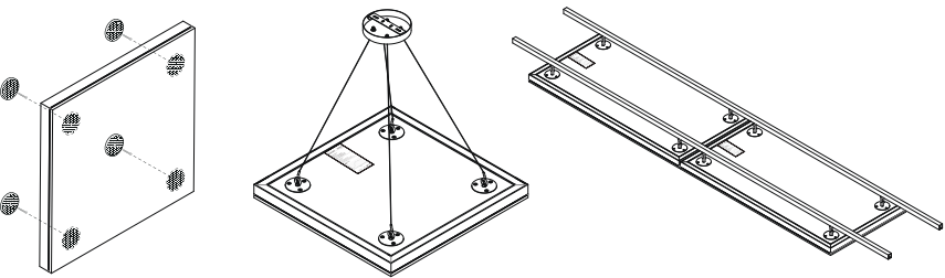
壁掛方式 Hanging installation diagram 單片吊裝 Hanging installation diagram 陣列吊裝 Hanging installation diagram
