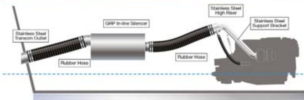
Dual Chamber Silencer with Above Water Discharge
