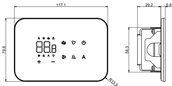
COMPACT i0912/i0924 VSD SMART - 3C0026254E / 3C0026255G
