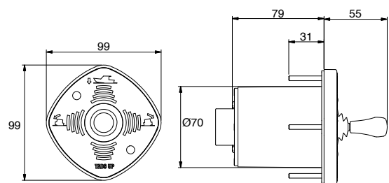
J/B-LED dimensions
