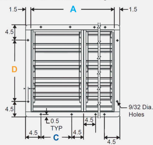
EASR Backdraft Shutter Air Entering Side
