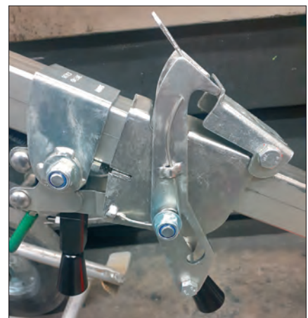
Double Drum Rim Locking Clasp
