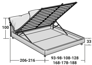
Misure interne vano contenitore: cm. 84/99/119/159/169/179/189x190/200x16,5h
