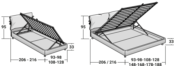
Misure interne vano contenitore: cm. 84/89/99/119/139/159/169/179x190/200x16,5 h
