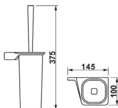
Belbagno Item Description AM-G-2739 Brush Holder
