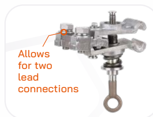
EFP-16705 CE20/2/A/S/RT EARTH CLAMP
