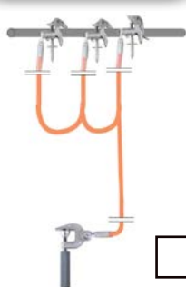
CONFIGURATION TYPE G
