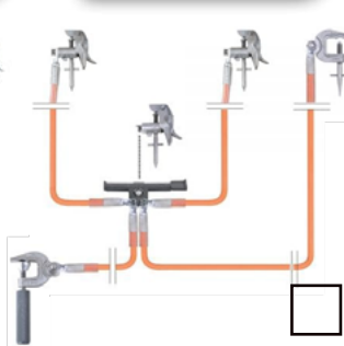
CONFIGURATION TYPE H
