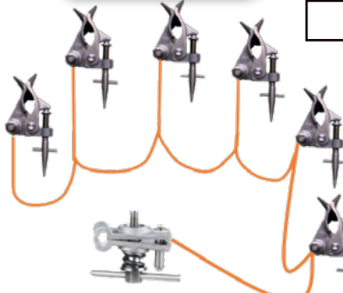
CONFIGURATION TYPE H
