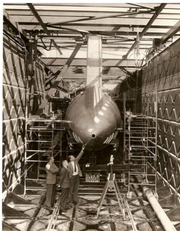
The Comet Test Tank with Walter (centre) and two colleagues. A Comet fuselage was mounted in the tank and repeatedly pressurised to represent a series of flights
