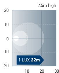
FMS1200 Light Distribution
