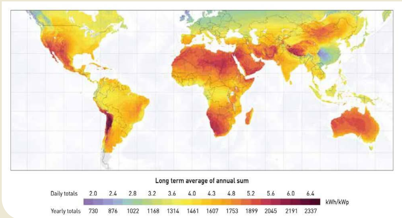
World Map of direct normal irradiation.
