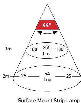
Surface Mount Strip Lamp
