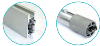
Beam 45 mm Ø 30 mm tube for LED frames
