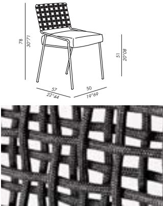
intreccio CHECKED - weave CHECKED
