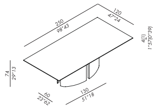
disegno piano metallo top design for metal finish
