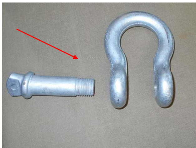
The Clevis Hook. TPDS-G12-220
