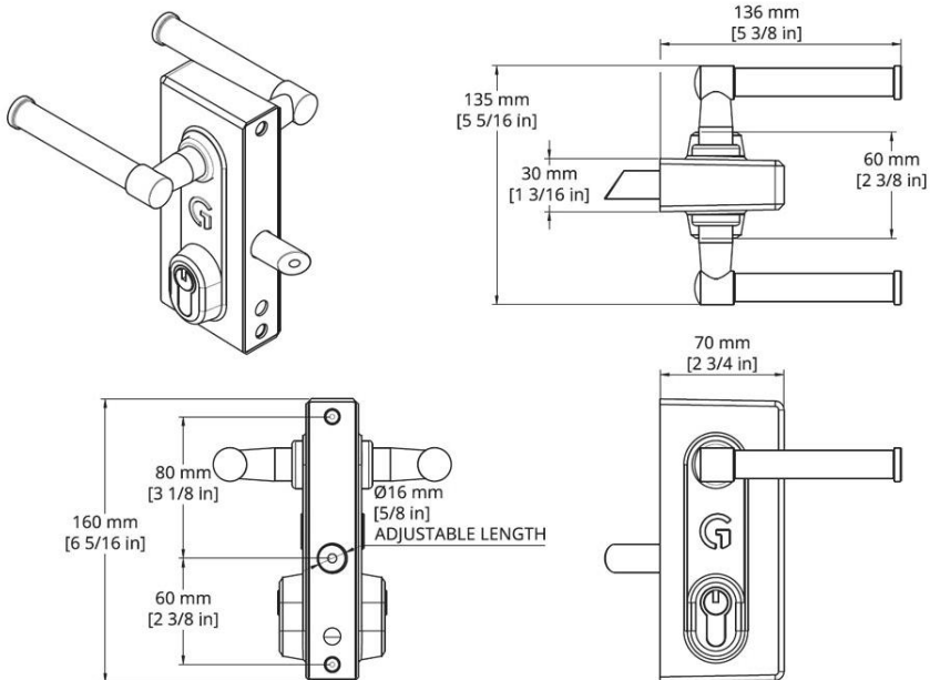
Dimension drawing:
