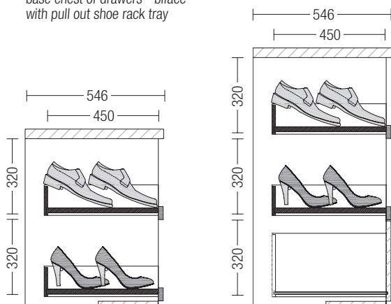
cassettiera base - bifacciale con vassoio portascarpe estraibile base chest of drawers - biface with pull out shoe rack tray
