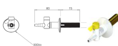
Ref: AM-900035 ONE WAY WALL MOUNTED DROP LEVER GAS TAP THREAD: 3/8 "
