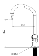
Ref: AM-900103 AM-900101 FIXED SWAN NECK WITH FIXED NOZZLE THREAD: 1/2 " BSP COLD (AM-900103) HOT (AM-900101)
