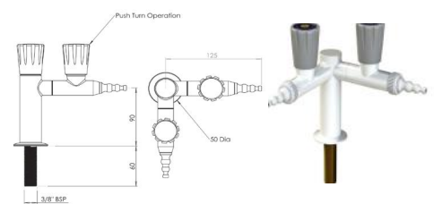
Ref: AM-900303 TWO WAY 90° BENCH MOUNTED GAS TAP WITH PUSH TURN HANDLE THREAD: 3/8 "
