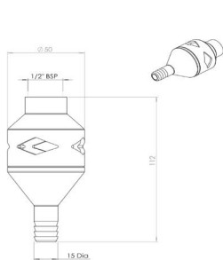
Ref: AM-900100 WRAS APPROVED BACK FLOW PREVENTION NOZZLE THREAD: 1/2 " BSP
