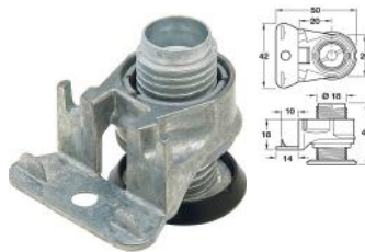
REF: AM-FOT002 ADJUSTABLE FOOT FOR LONG ALIGNING HEAVY FURNITURE, INTEGRATO G HEIGHT ADJUST LOAD RATING 25 MM 175 KG
