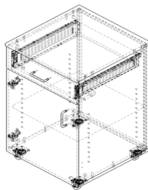
Mobile Single Drawlined Cupboard Left Hand Hinged Door Ref: AM-LAB-MSCDL
