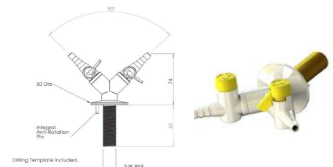
Ref: AM-900036 TWO WAY WALL MOUNTED DROP LEVER GAS TAP THREAD: 3/8 "
