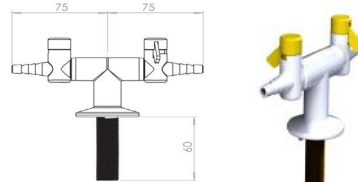
Ref: AM-900032 TWO WAY 180° BENCH MOUNTED DROP LEVER GAS TAP THREAD: 3/8 "
