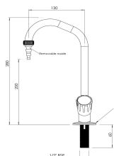
Ref: AM-902103 AM-902101 FIXED SWAN NECK WITH REMOVABLE NOZZLE THREAD: 1/2 " BSP COLD (AM-902103) HOT (AM-902101)
