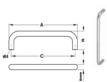
Ref: AM-HAN221 CLIFTON STAINLESS STEEL BOW HANDLE LENGTH 184 MM (A) HOLE SPACING 160 MM (C) DEPTH 32 MM (B) FINISH BRUSHED EFFECT
