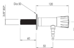
Ref: AM-900198 WALL MOUNTED STAINLESS STEEL WATER TAP FOR SPECIAL WATERS THREAD: 3/8 " BSP
