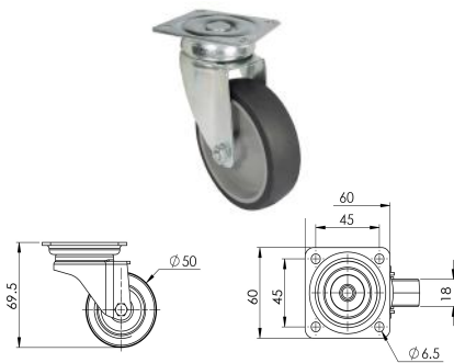
REF: AM-CST001 DIAMETER WHEEL WIDTH LOAD CAPACITY COLOUR CASTOR-2" SCREW IN RUBBER CASTOR - GREY UNBRAKED 50.0 MM / 1.969" 18 MM 40KG BLACK
