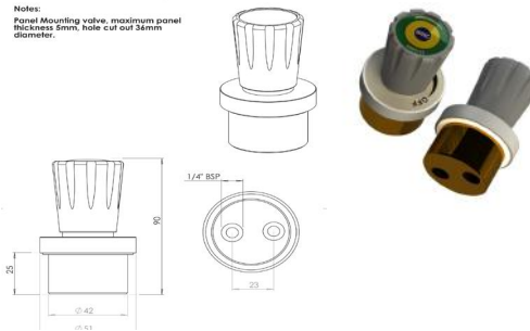
Ref: AM-901711 FRONT CONTROL VALVE FOR A VARIETY OF SERVICES THREAD: 1/4 " BSP
