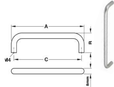
Ref: AM-HAN121 D PULL HANDLE LENGTH 168MM (A) HOLE SPACING 160MM (C) DEPTH 30MM (B) FINISH ALUMINIUM
