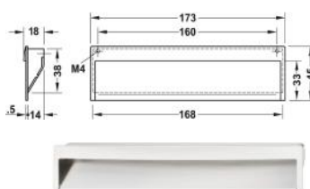
Ref: AM-HAN411 FLUSH ZINC ALLOY HANDLE LENGTH 173 MM HOLE SPACING 160 MM HEIGHT 45 MM DEPTH 18 MM FINISH BRUSHED NICKEL
