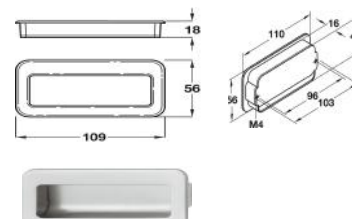
Ref: AM-HAN421 FLUSH ZINC ALLOY HANDLE LENGTH 109MM HOLE SPACING 96 MM HEIGHT 56 MM DEPTH 18MM FINISH BRUSHED CHROME
