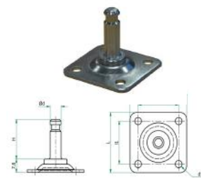
REF: AM-CST012 DIAMETER LOAD CAPACITY COLOUR 2" CASTOR PLATE FIXING 50.0 MM / 1.969" 60KG BLACK
