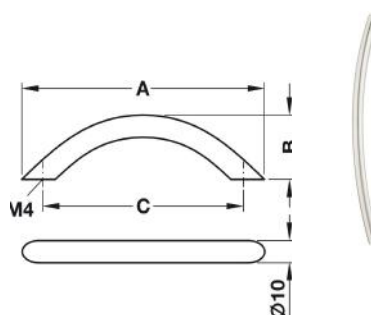
Ref: AM-HAN221 CLIFTON STAINLESS STEEL BOW HANDLE LENGTH 184 MM (A) HOLE SPACING 160 MM (C) DEPTH 32 MM (B) FINISH BRUSHED EFFECT
