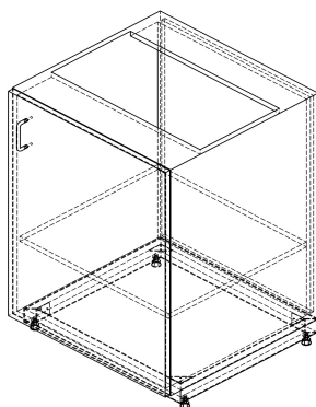
Fitted Single Cupboard Right Hand Hinged Door
