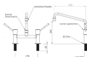
Ref: AM-910078 H PATTERN MIXER TAP WITH LEVER ACTION AND AERATOR NOZZLE THREAD: 1/2 " BSP
