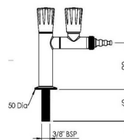
Ref: AM-902503 2 WAY DRY SERVICE TAP WITH REMOVABLE NOZZLE THREAD: 3/8 " BSP
