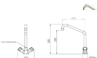
Ref: AM-900115 MONOBLOCK MIXER WITH AERATOR THREAD: 1/2 " BSP
