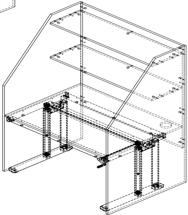
Write-up Desk Height Adjustable
