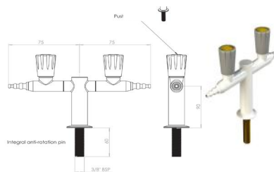
Ref: AM-900302 TWO WAY 180° BENCH MOUNTED GAS TAP WITH PUSH TURN HANDLE THREAD: 3/8 "
