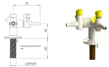
Ref: AM-900033 TWO WAY 90° BENCH MOUNTED DROP LEVER GAS TAP THREAD: 3/8 "
