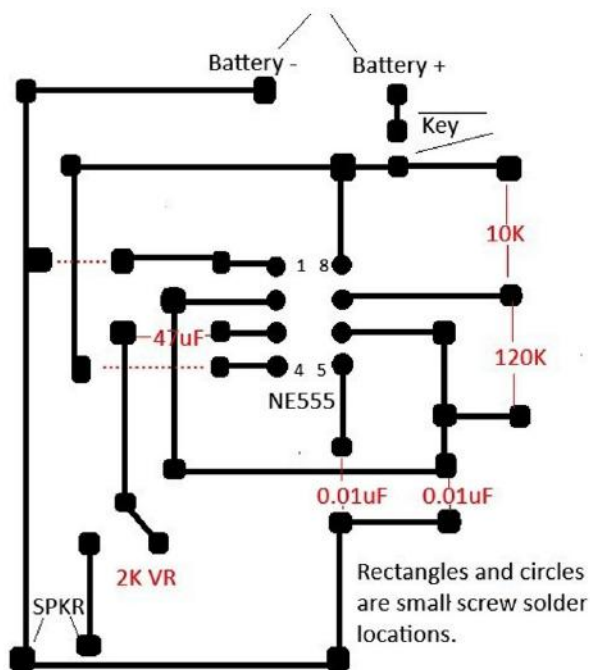
Schematic Diagram of Morse Practice Oscillator
