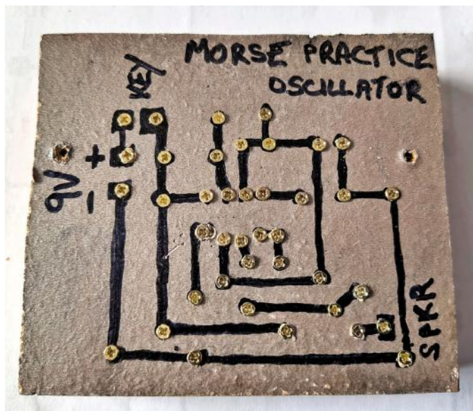
Circuit Traces with Screws Inserted
