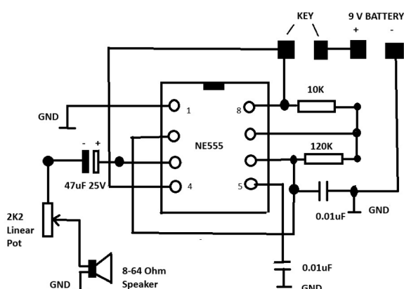
Schematic Diagram of Morse Practice Oscillator
