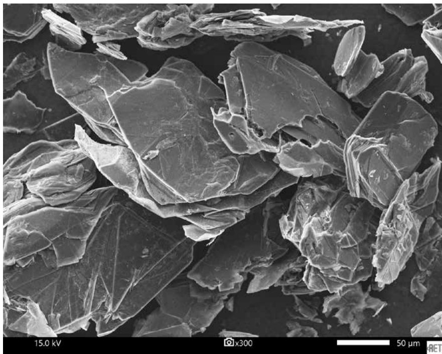
Concentré de graphite naturel en paillettes de Lac Knife de Focus Graphite. / Focus Graphite Lake Knife natural flake concentrate.
