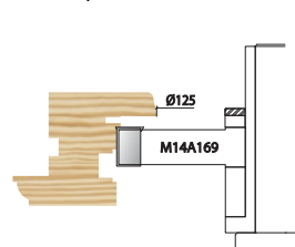
Sash Top/Bottom Rail
