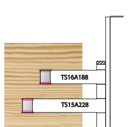
Frame Comb Joint Slots
