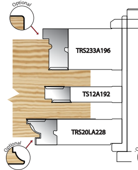
Frame Comb Joint Scribe
