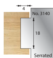
Cutter: 003SH03140 Limiter: 004SH03140
