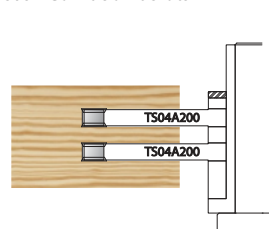
Sash Comb Joint Slots
