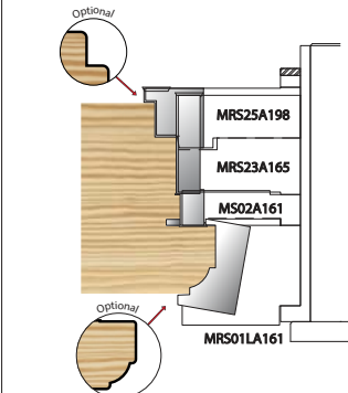
Frame Mould Cill
