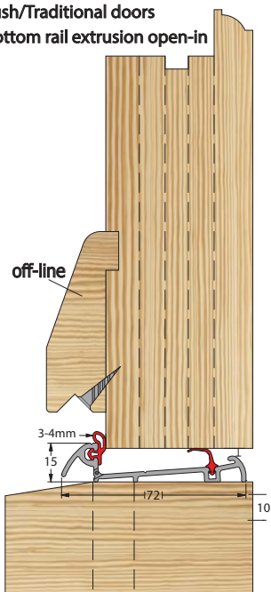
Tooling Set D3
