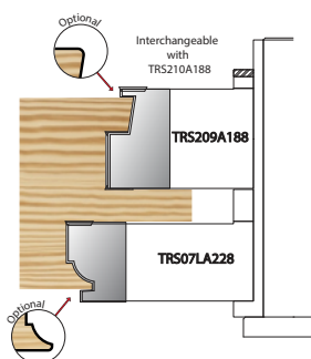
Frame Single Tenon Scribe Cill
