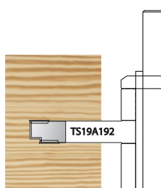
Frame Single Tenon Slot
