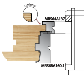
Sash Outside Mould (Head & Lock)
