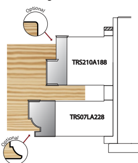
Frame Single Tenon Scribe
