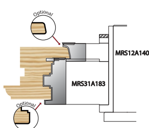
Sash Outside Mould
