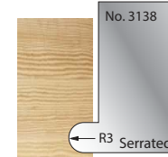
Cutter: 003SH03138 Limiter: 004SH03138
