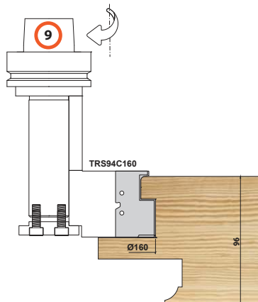
Frame Rebate Tenon Scribe
