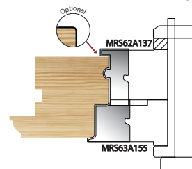
Sash Outside Mould (Butt Hinge)
