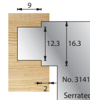
Cutter: 003SH03141 Limiter: 004SH03141
