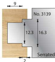
Cutter: 003SH03139 Limiter: 004SH03139
