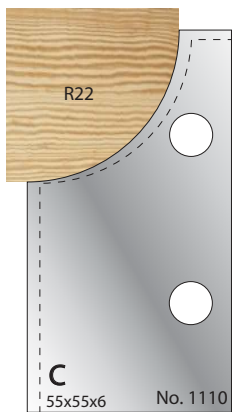
Cutter: 003H01110 Limiter: 004H01110
