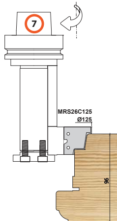
Frame Mould Cill
