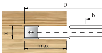
150 x 4 - 7.5 Adj. TB Groover (2 part)
