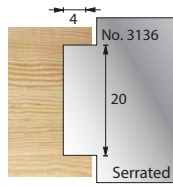
Cutter: 003SH03136 Limiter: 004SH03136
