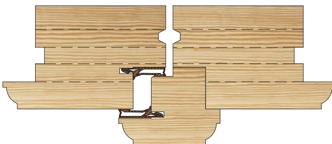
French doors meeting stiles
