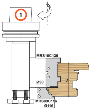
Sash Inside Mould
