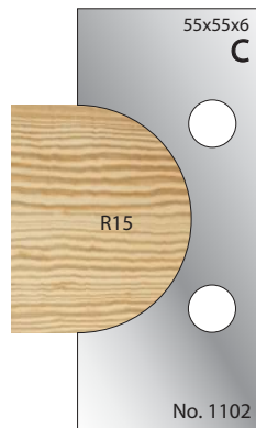
Cutter: 003H01102 Limiter: 004H01102
