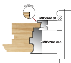
Sash Outside Mould (Cill)
