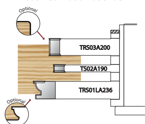
Sash Comb Joint Scribe
