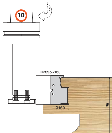
Frame Rebate Tenon Scribe Cill
