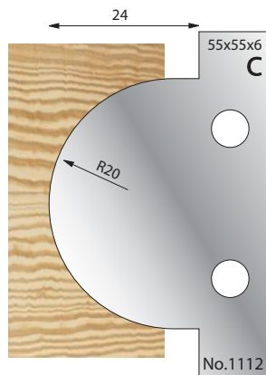
Cutter: 003H01112 Limiter: 004H01112
