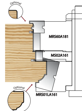
Frame Mould Cill
