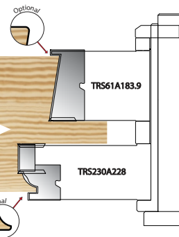
Frame Single Tenon Scribe Cill
