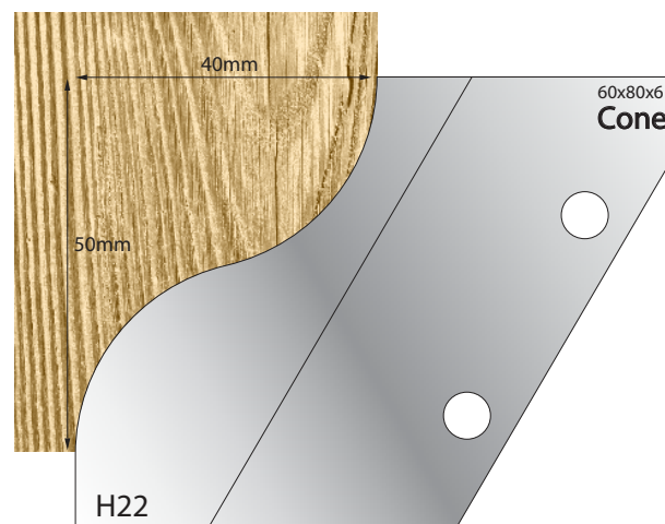
Cutter: 003H00H22 Limiter: 004H00H22
