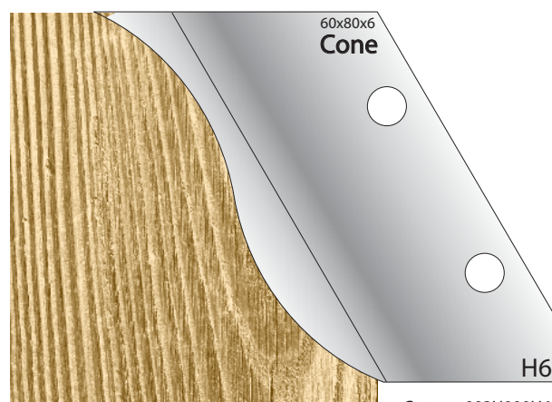
Cutter: 003H000H6 Limiter: 004H000H6
