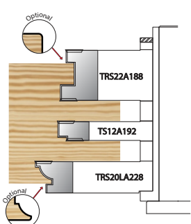
Frame Comb Joint Scribe
