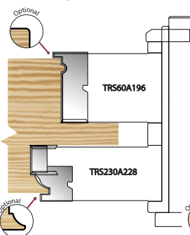
Frame Single Tenon Scribe
