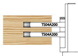
Sash Comb Joint Slots
