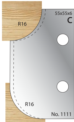
Cutter: 003H01111 Limiter: 004H01111
