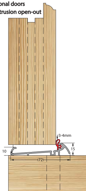
Tooling Set D4
