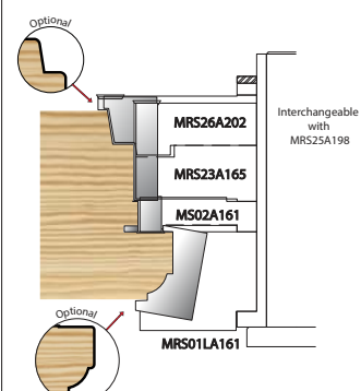
Frame Mould Cill
