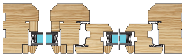
BB Horizontal
