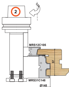
Sash Outside Mould
