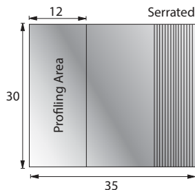
Cutter: 003SH03139 Limiter: 004SH03139
