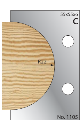
Cutter: 003H01105 Limiter: 004H01105
