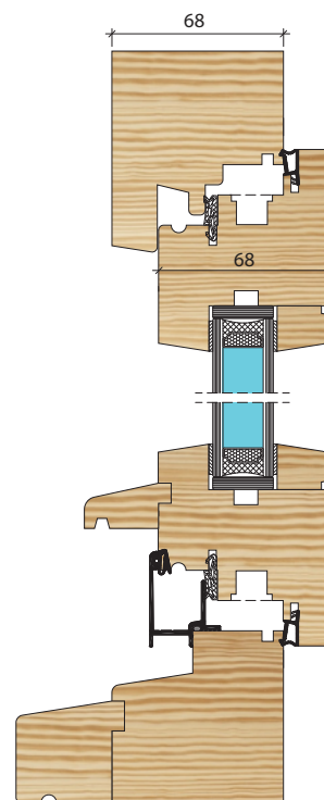
Vertical Sections
