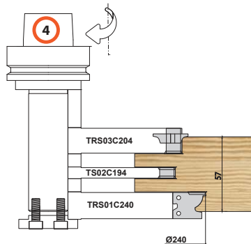
Sash Comb Joint Scribe
