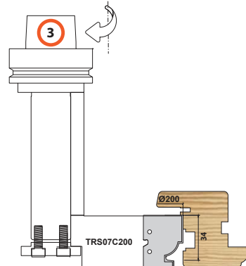
Sash Top/Bottom Rail
