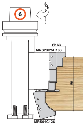
Frame Mould
