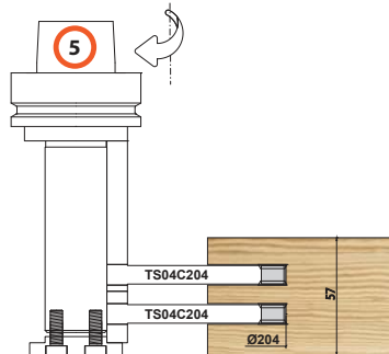
Sash Comb Joint Slots
