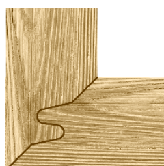
Horizontal cut 15/28mm material
