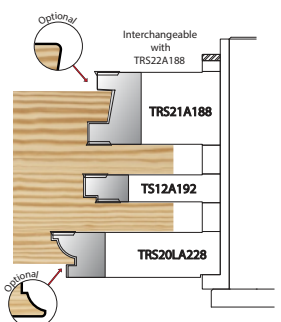
Frame Comb Joint Scribe Cill
