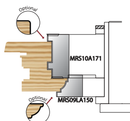
Sash Inside Mould
