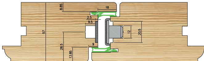
French Doors Meeting Stiles for Double Handle - KLONE (Page 126)
