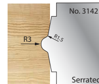
Cutter: 003SH03142 Limiter: 004SH03142
