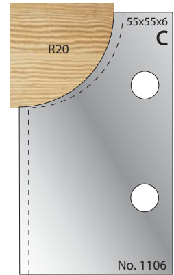
Cutter: 003H01106 Limiter: 004H01106
