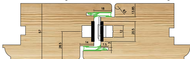
French Doors Meeting Stiles for Double Handle - KLONE (Page 126)
