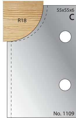
Cutter: 003H01109 Limiter: 004H01109
