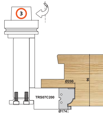
Frame Profile Tenon Scribe
