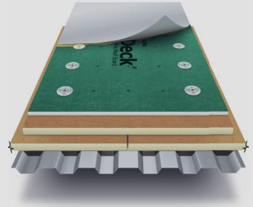
Above: With its enhanced gypsum core, coated face and back glass mats, DensDeck Prime Roof Board acts as a durable cover board and mitigation layer within the roof assembly.
