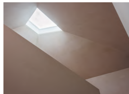
Above: Internally the frameless design of the bespoke rooflights maximises daylight.
