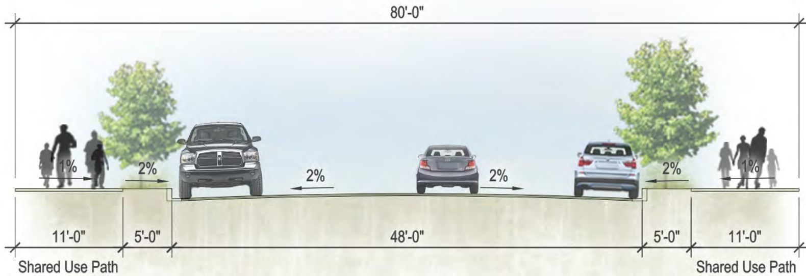
Trails Along Collector Roads: Recommended Standard Modification Scale: 1" = 10'
