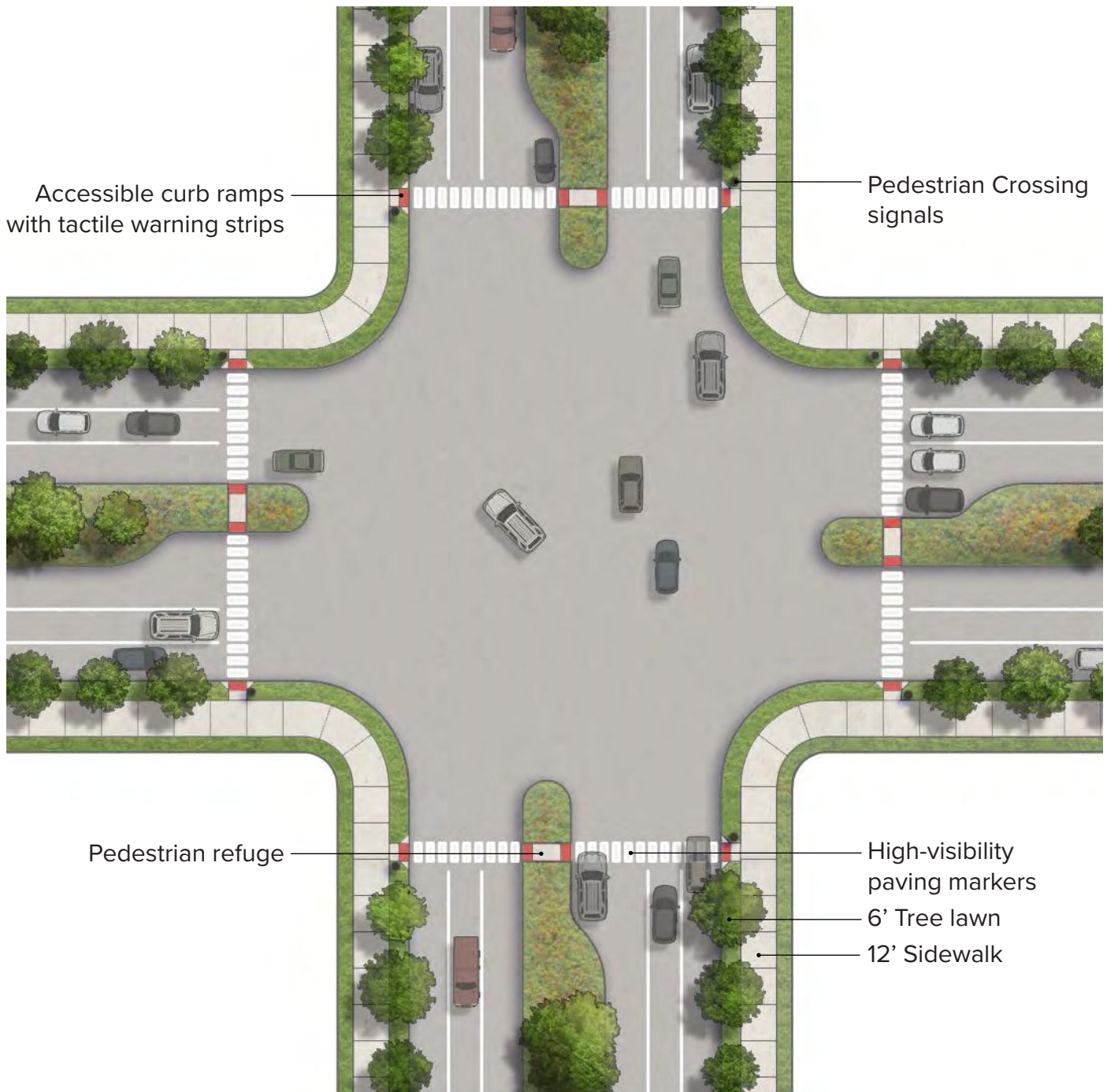
Safe Crossing Standards: Crosswalk with Pedestrian Refuge Scale: 1" = 50'
