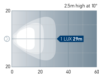
Sea Hawk-XL Dual Colour - Spread
