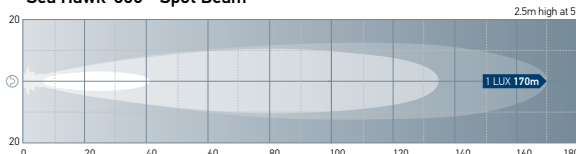
Sea Hawk-350 - Spot Beam
