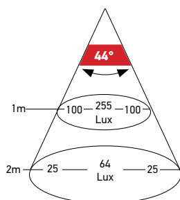
Surface Mount Strip Lamp
