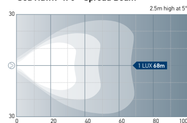
Sea Hawk-470 - Spread Beam
