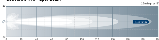
Sea Hawk-470 - Spot Beam
