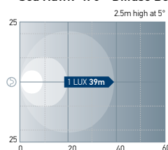
Sea Hawk-470 - Diffuse Beam
