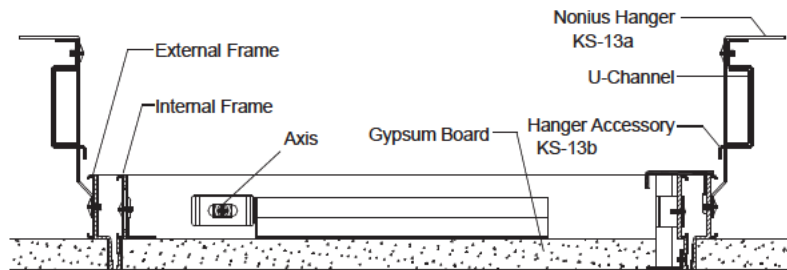
FIG. B Installation Drawing of KIJH Hatch
