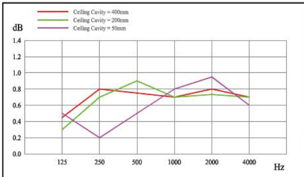
FIG.B: The Sound Absorption Performance Range
