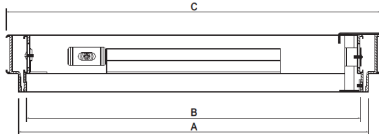
FIG. A Section Drawing of KIJH Hatch
