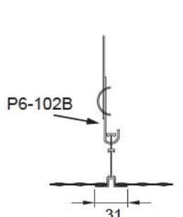
Mesh ceiling panel
