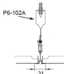
Lay-on ceiling panel
