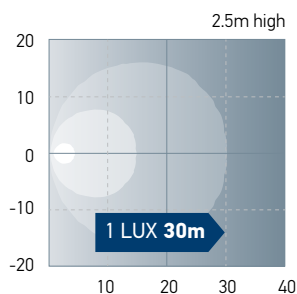
FMS2500 Light Distribution
