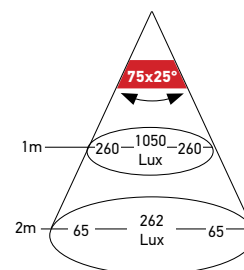
Sea Hawk Dual Color
