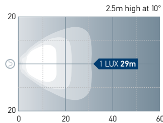
Sea Hawk-XL Dual Color - Spread
