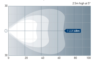
Sea Hawk-470 - Spread Beam
