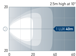
Sea Hawk-XLR - Spread
