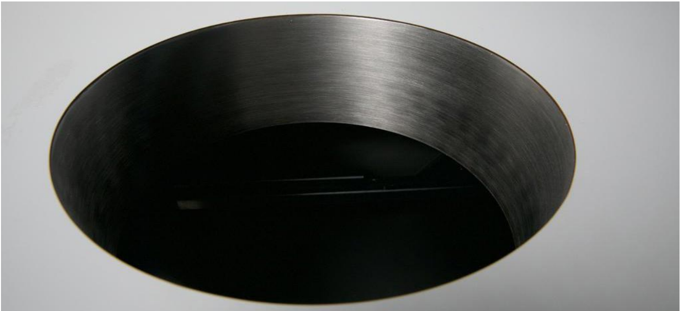
Circular Waste Chute Cabinet Size 300 mm Overall Size Dia. 200 x H80 mm Main Bowl Size Dia. 150 x H80 mm Stainless Steel Satin, Grade 304 Stock Code WCFE-D150 Circular Waste Chute
