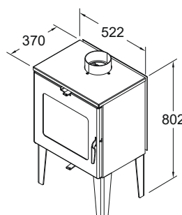
VisionLine s35-1 (uten sideglass)
