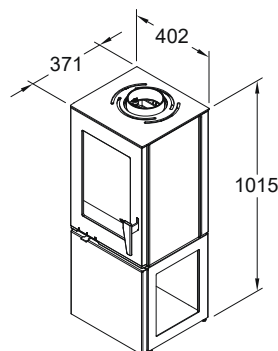
VisionLine s40-1 (uten sideglass)
