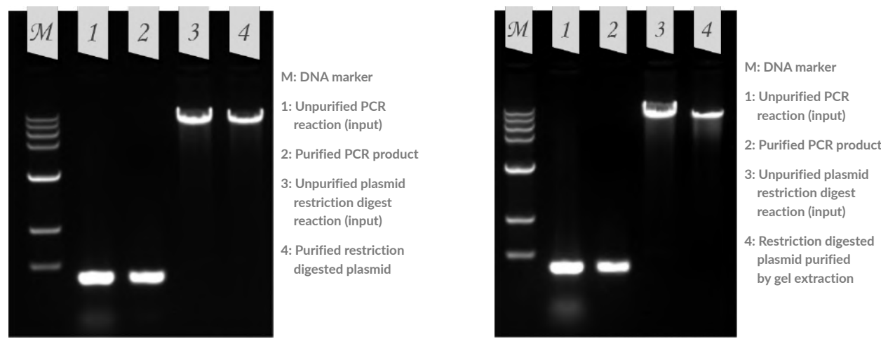
Agarose gel electrophoresis of PCR-purified DNA (left) and gel extracted-DNA (right) using SPINeasy PCR Purification and Gel Extraction Kit
