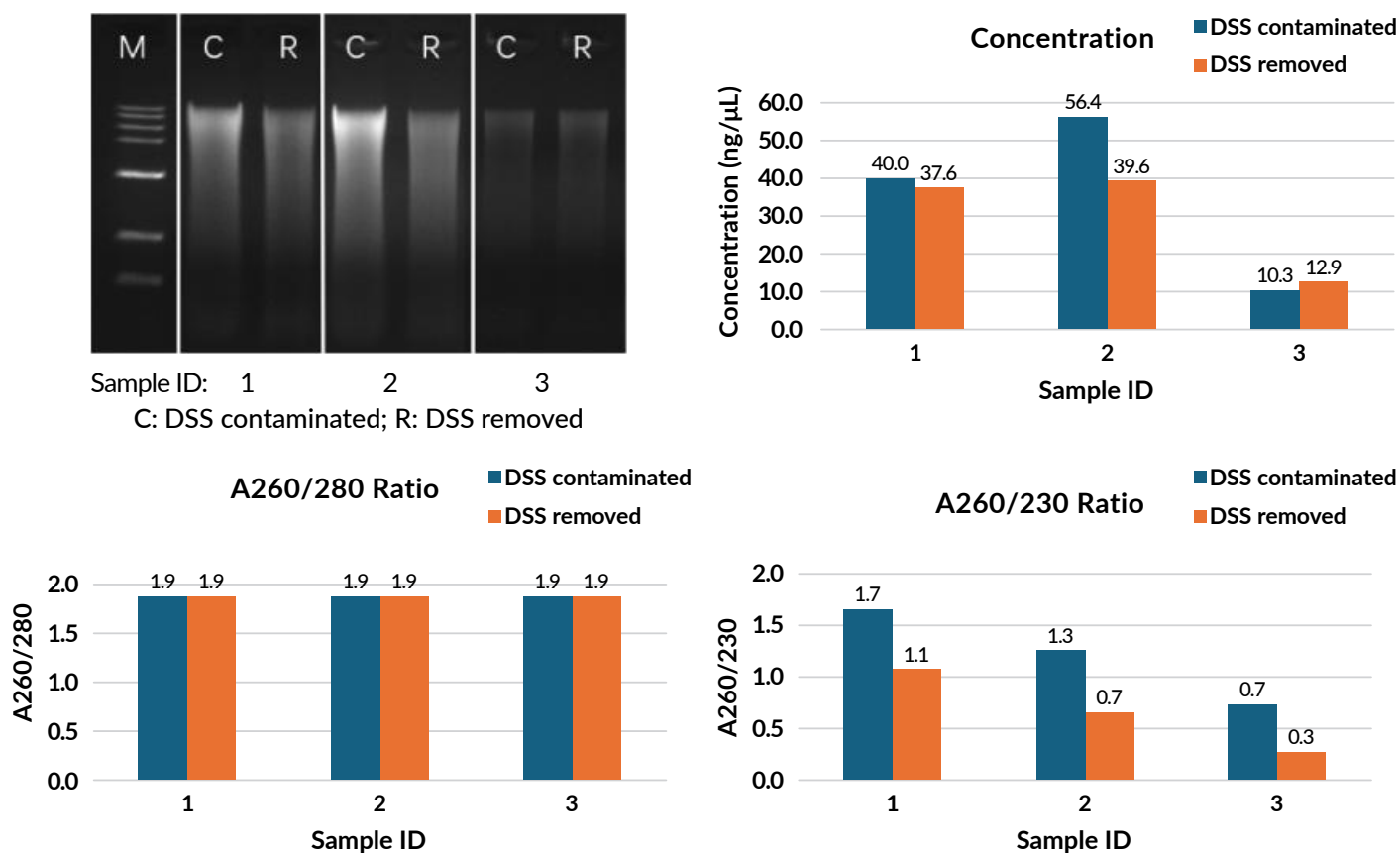
Figure 1: DNA yield and purity (A260/A280 and A260/A230 ratios) obtained from mouse feces (sample 1&2) and mouse intestinal contents (sample 3) using the SPINeasy DSS-Removal DNA Kit for Feces. The impact of DSS removal on DNA yield and purity may vary depending on the sample type, but remains consistently positive.
