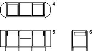
Interior View 4.plan 5.front 6.side
