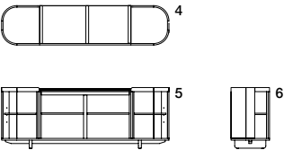
Interior View 4.plan 5.front 6.side
