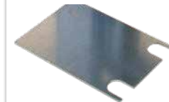
M70 Shim (100x100x1.2mm)
