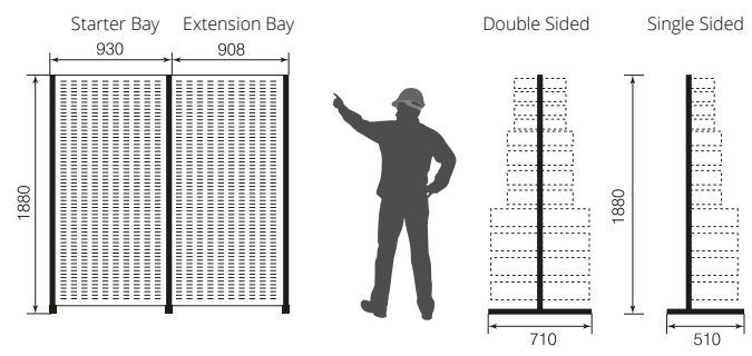
Louvre Rack dimensions (mm)
