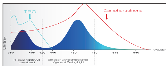
O-Light Plus Spectral Curve & Resin Spectral Absorptivity
