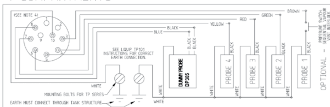
Wiring Diagram for a 4 Compartment Tanker using a 6 Channel Monitor
