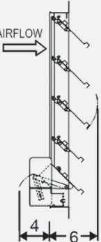
EASR Motor Operated Single Panel
