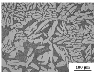
OM micrograph of heat-treated L-PBF-Ti64
