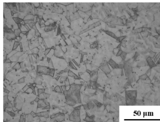
OM micrograph of annealed 316L Stainless Steel
