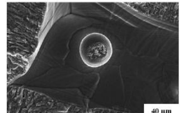
Fracture Surface of L-PBF-Ti64
