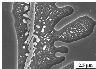
SEM micrograph of Bronze
