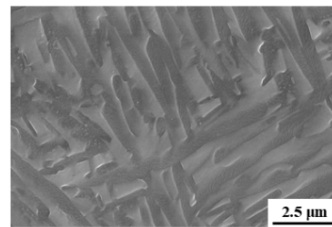
SEM micrograph of heat-treated L-PBF-Ti6242
