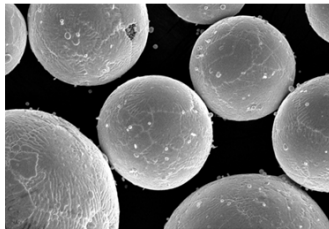
SEM micrograph of C103 powder particles
