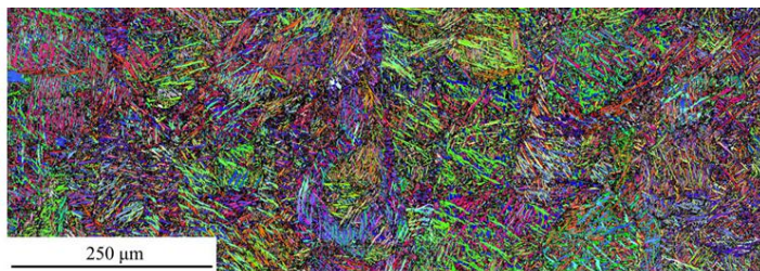
EBSD of L-PBF-Ti6242
