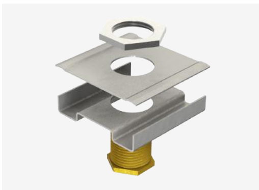
50 x 50mm Lighting Trunking Suspension Unit
