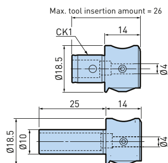
Head EWN04-7 Stroke -0.1 - +1.05mm
