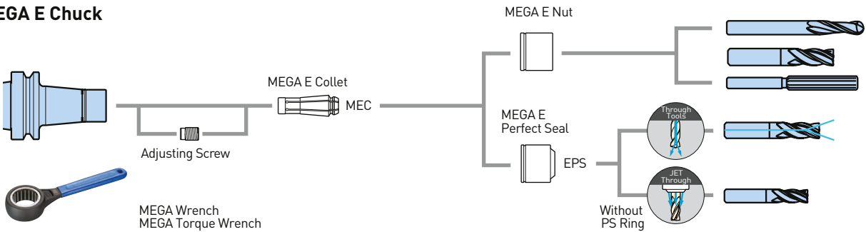
MEGA E Perfect Seal
