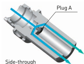
Side-through
