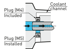
Center Through
