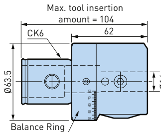
Head EWB2-50CK6
