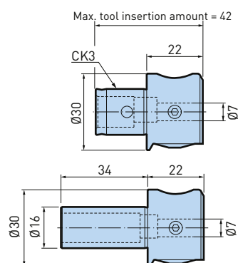
Head EWN04-15 Stroke -0.2 - +2.0mm
