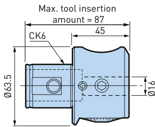
Head EWN2-54CK6
