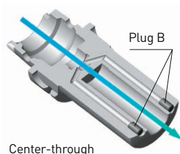
Center-through
