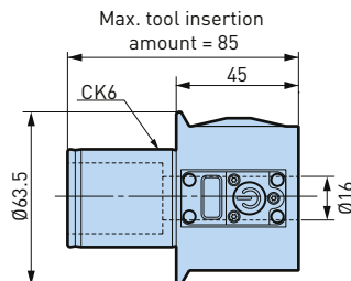
Head EWE2-54CK6
