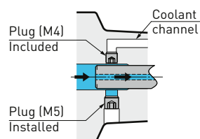
Center Through
