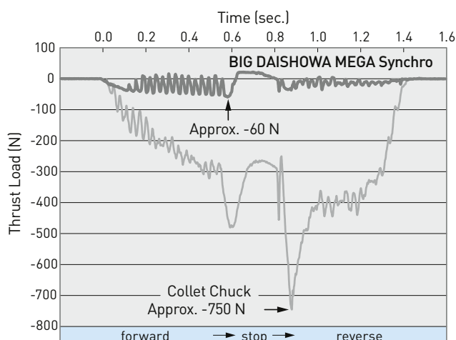
Collet chuck
